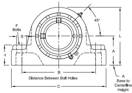
Fixed Block
