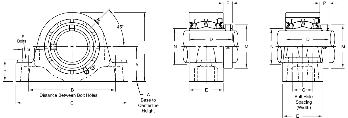
Fixed Block
