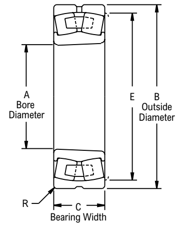
Tapered Bore
