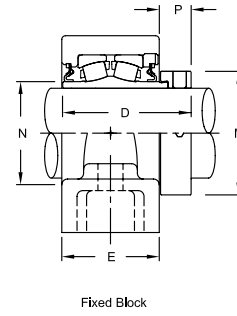
Fixed Block
