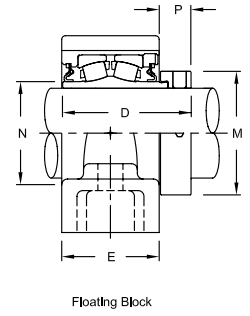
Floating Block
